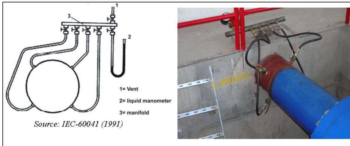
Fig. 10 : Pressure taps connected through separate connecting pips to box-type manifold
